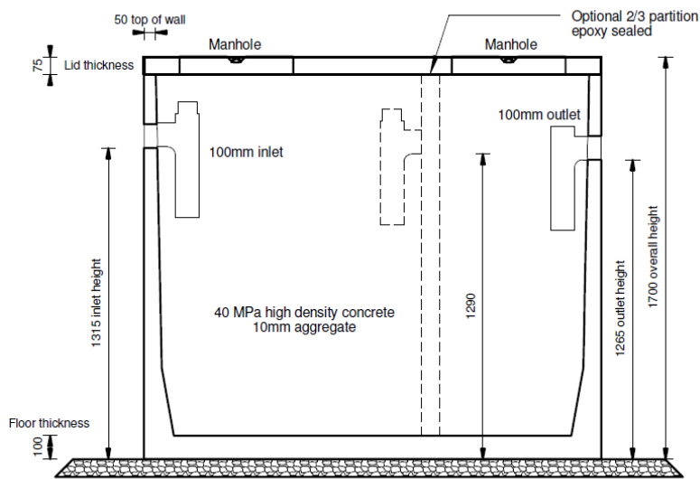
2.5m x 2.5m leveled site with 75mm of 10mm scredded gravel
